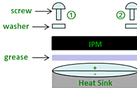
Figure 8. Mounting Composition
