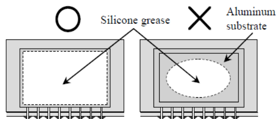
Figure 10. Grease Application
